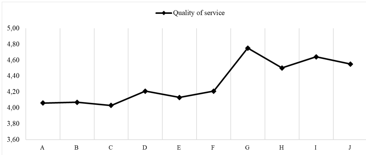
Graph 1. Mean of the latent variable quality
